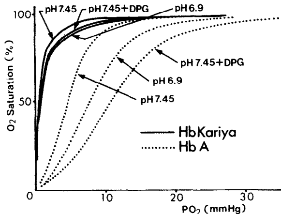
Fig. 2. Oxygen dissociation curves of Hb Kariya and Hb A.
